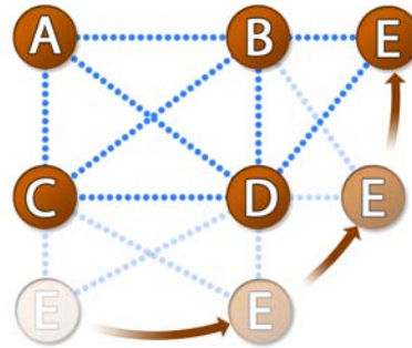
Figure 8. The Rajant mesh network quickly adapts to the changes caused by the movement of Node E. New resilient links are established in real-time.
